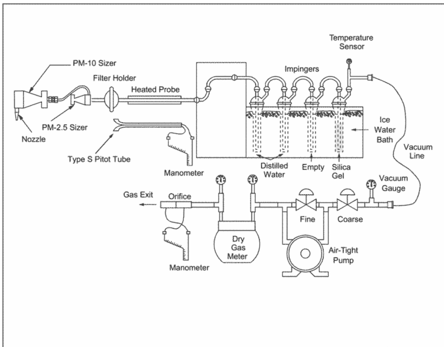
Figure 1. In-stack PM_{10} and PM_{2.5} Sampling Train
