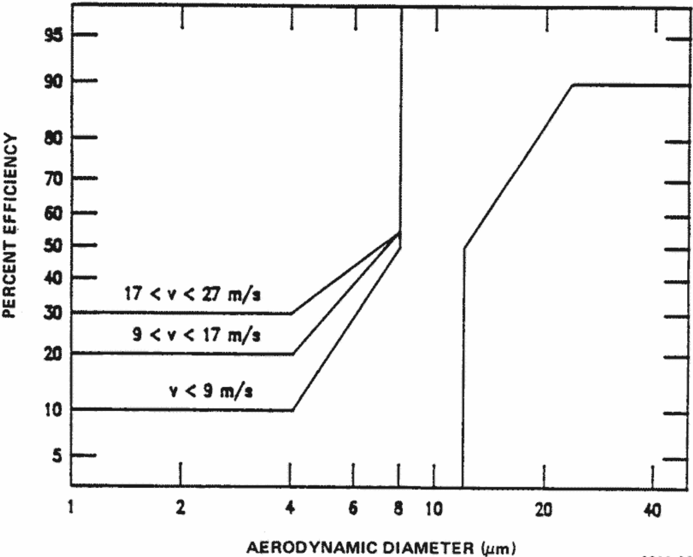
Figure 13. Efficiency envelope for the PM 10 cyclone.
