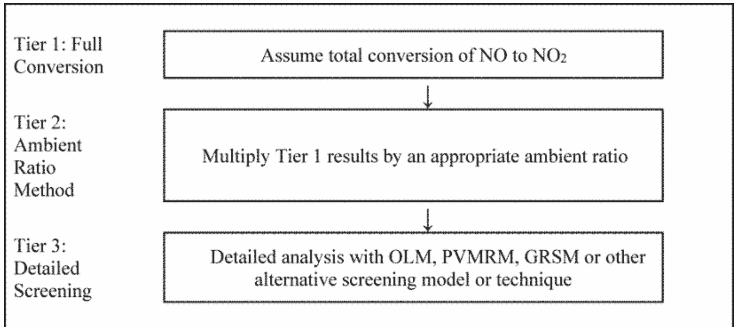
Figure 4-1: Multi-Tiered Approach for Estimating \text{NO}_2 Concentrations
