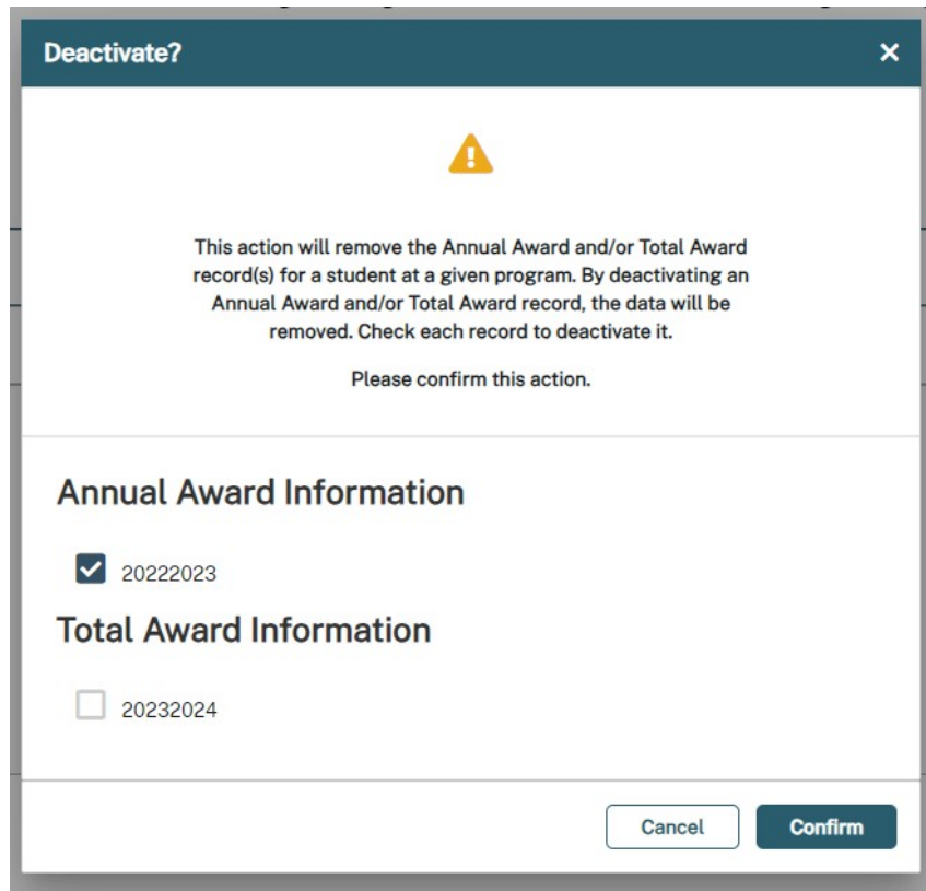
Figure 34: Deactivate? Popup
