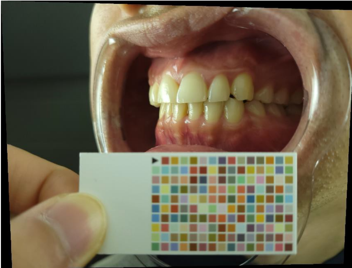
Permanent molars
