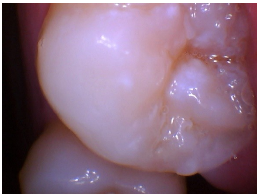
1 st molar
