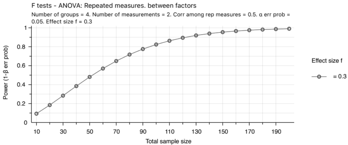
Figure 4. Expected statistical power as a function of total sample size for a repeated measure, between-factors ANOVA with an assumed low-medium effect size of 0.3.
