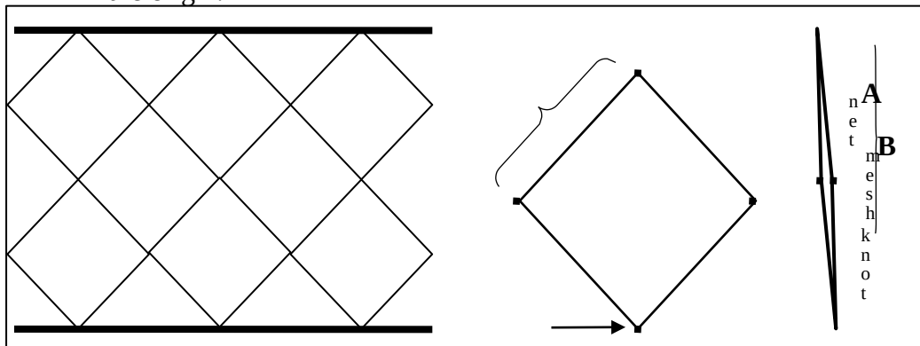
Figure 2. Typical net design. Nets are measured by the depth and length of the meshes between
